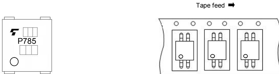
Figure1 Device Orientation
