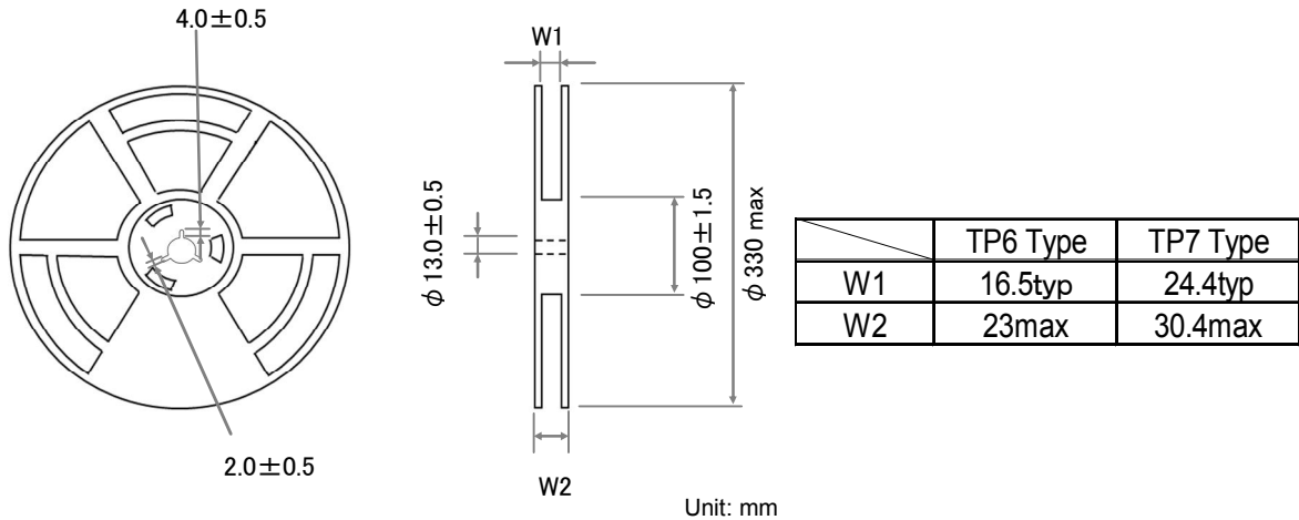
Figure 4 Reel Forms
